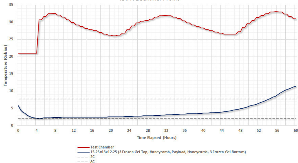
ColdCorr 15.25x13x12.25 Summer Testing ISTA 7E Summer Profile
